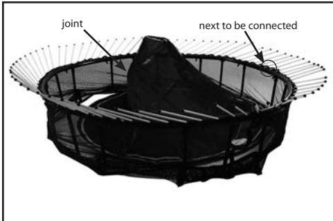
Figure 11-A: Attaching the mat to the rods
