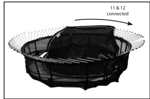
Figure 12-A: Attaching the next (eleventh and twelfth) rods
