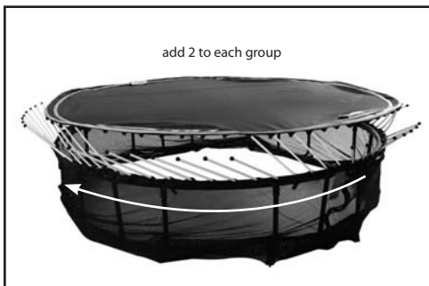
Figure 14-A: Adding 2 rods per group
