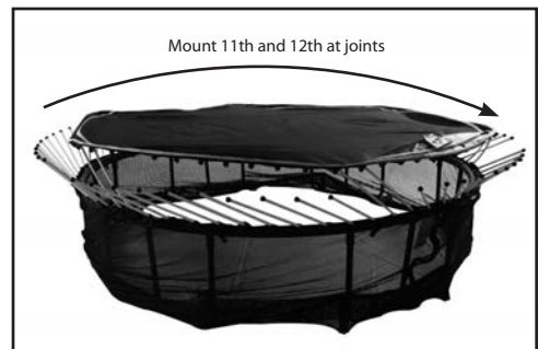
Figure 13-A: Every eleventh and twelfth rod attached
