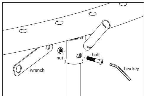
Figure 6: Fastening the last three legs
