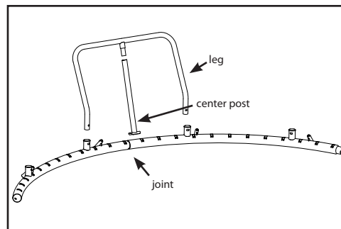
Figure 2-A: Inserting a leg piece and center post
