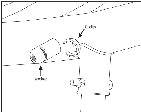
Figure 20: C-clip attached to socket on frame
