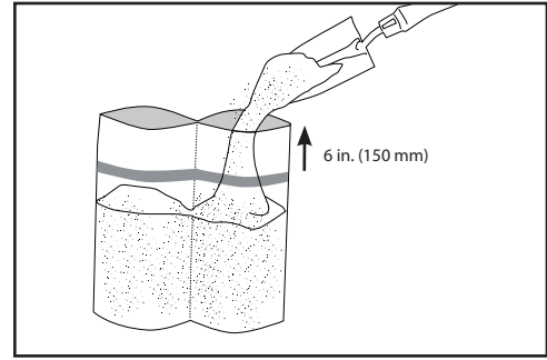
Figure 21-A: Filling the sandbag
