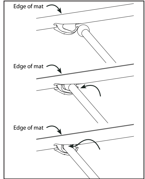
Figure 11-B: Fitting the mat rod into the mat edge socket
