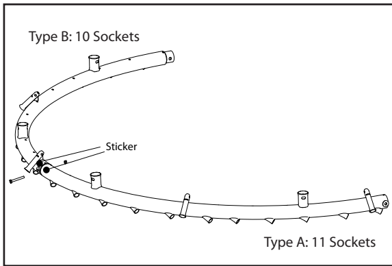
Figure 2-C: Fastening curved frame sections
