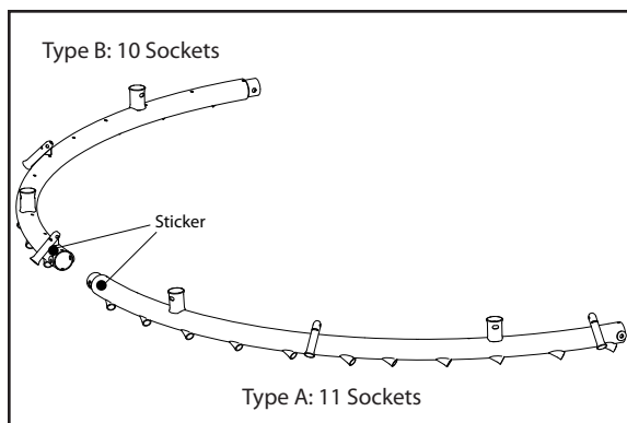
Figure 2-B: Joining curved sections
