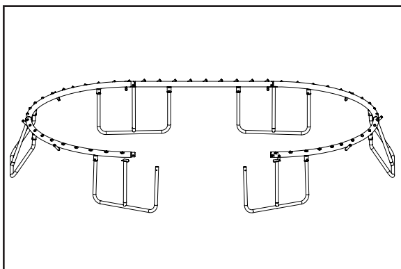
Figure 5-E: Attaching straight frame section onto half circle frame sections
