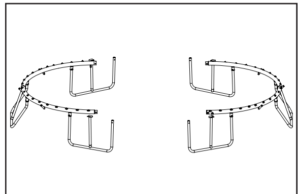
Figure 5-C: Attaching remaining legs
