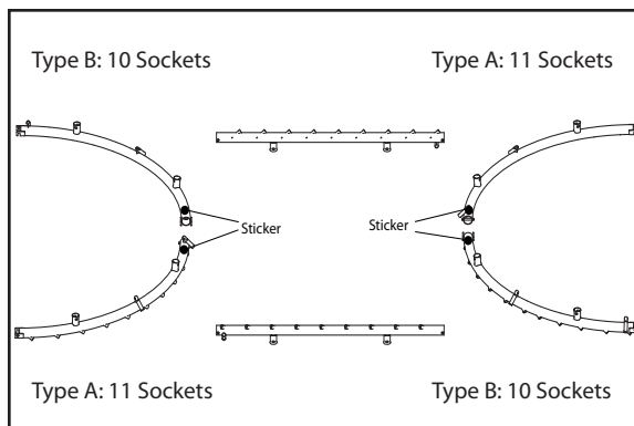
Figure 2-A: Laying out the frame sections
