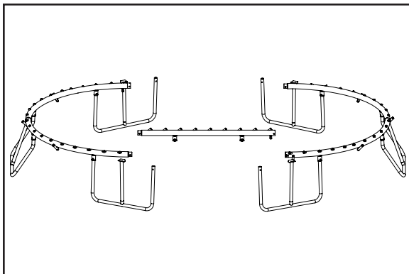
Figure 5-D: Adjusting spacing for straight section
