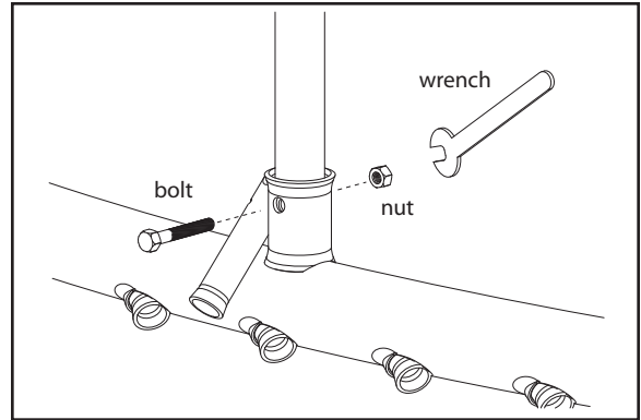
Figure 4-B: Fastening the legs to the frame
